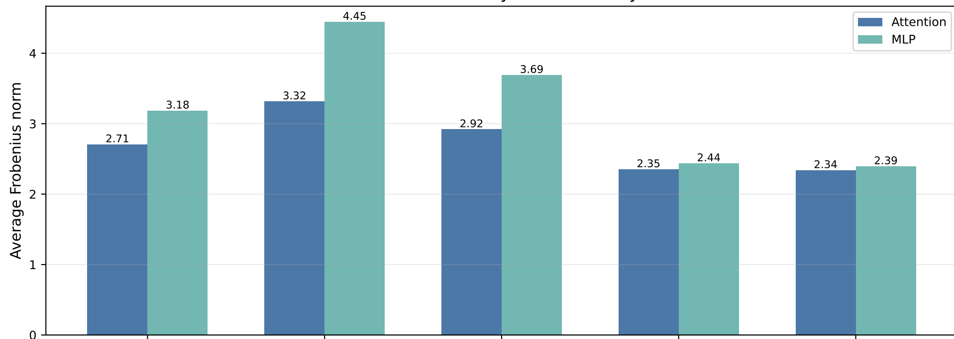
LoRA B norms by module family
