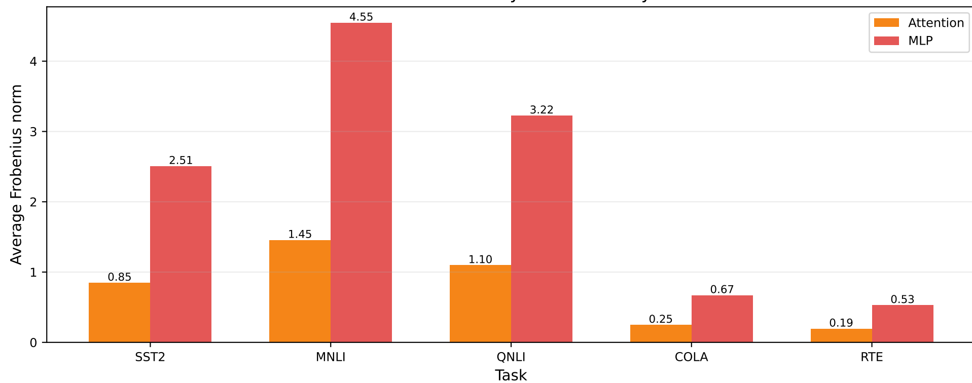
LoRA B norms by module family
